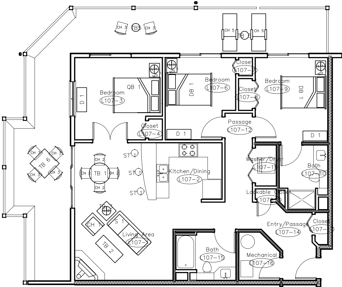
Floor Plan F - Units 107, 207, 307
